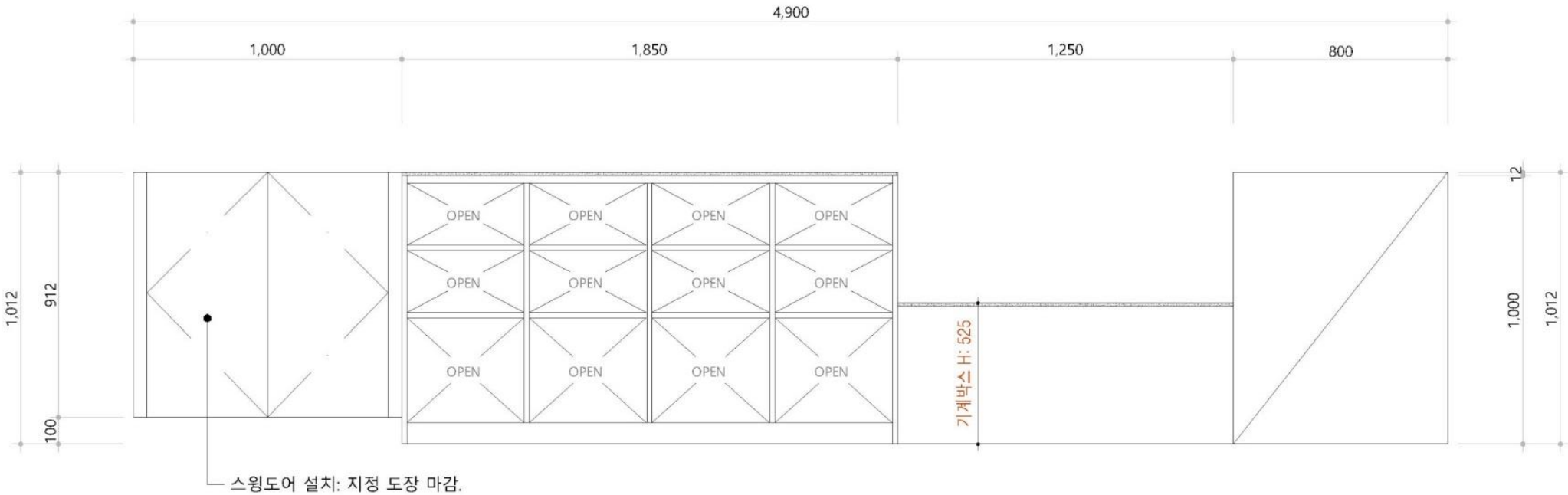
ELEVATION C
