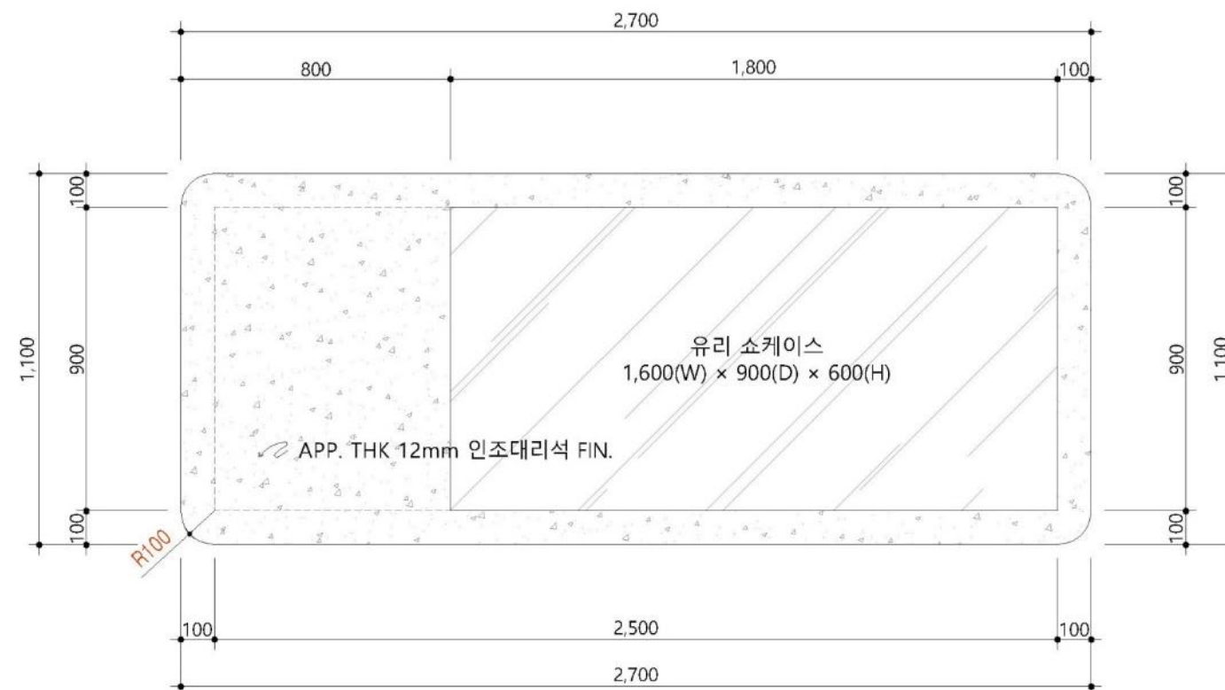
TOP VIEW
