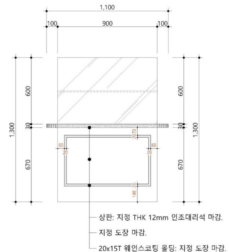
SIDE VIEW
