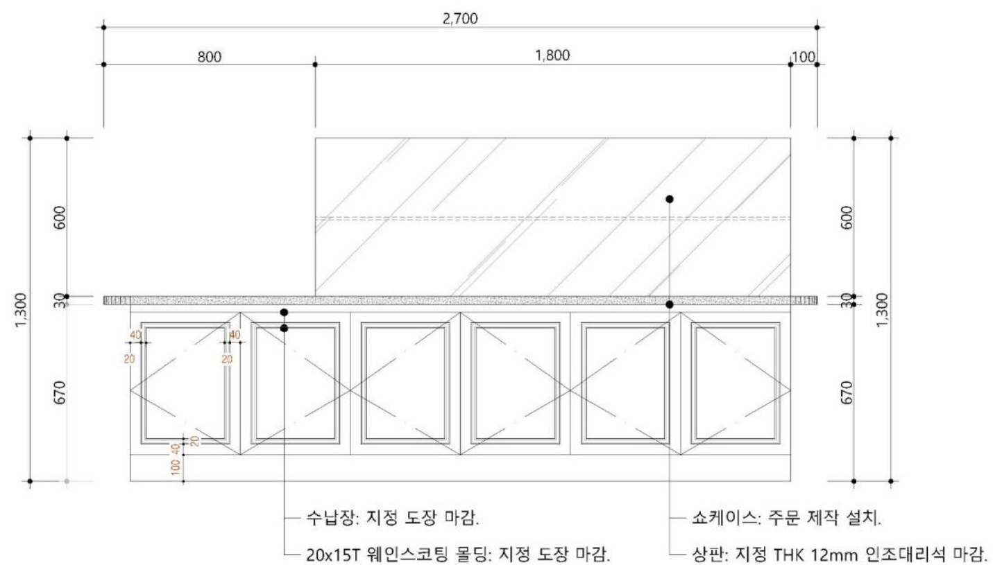
PRONT VIEW
