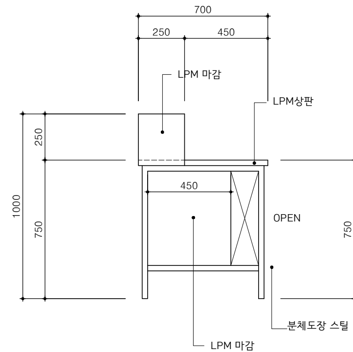
SECTION "A" SCALE : 1 / 20
