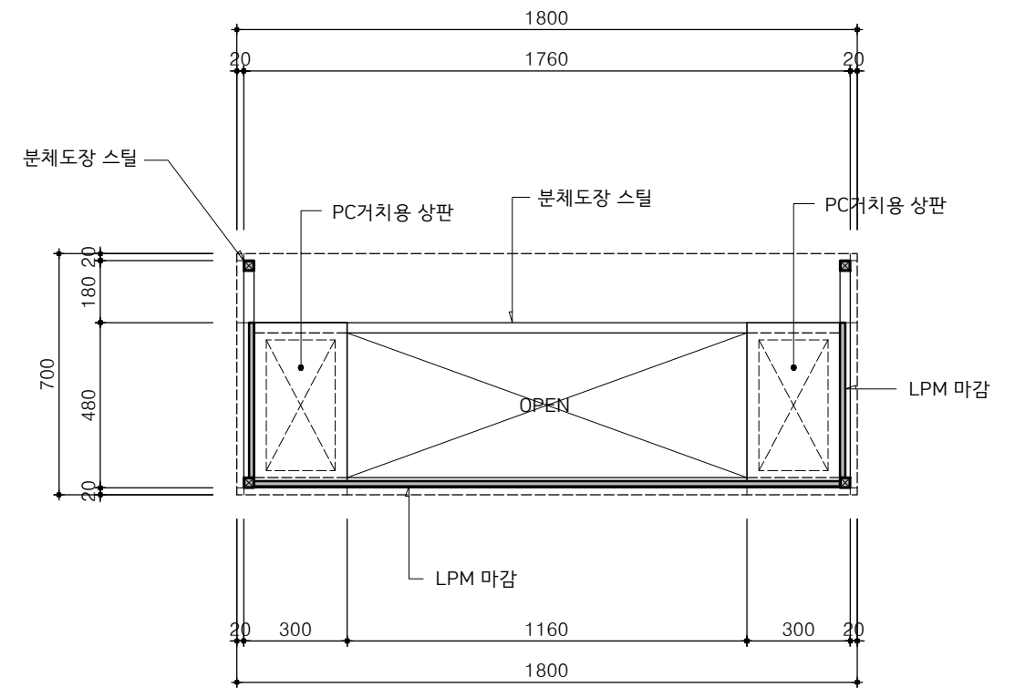
SECTION "A" SCALE : 1 / 20
