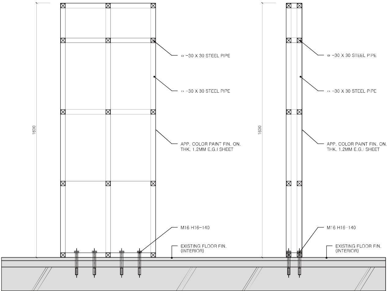
1 FRONT SECTION SCALE : 1/NONE
