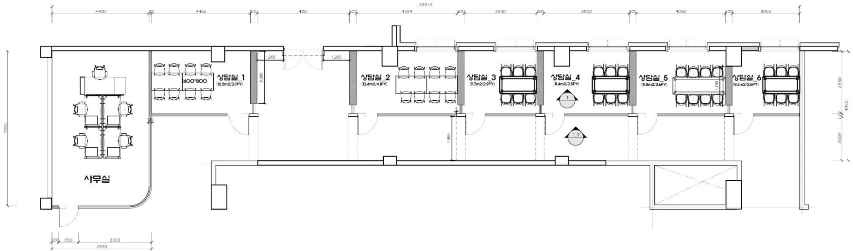
FLOOR PLAN
