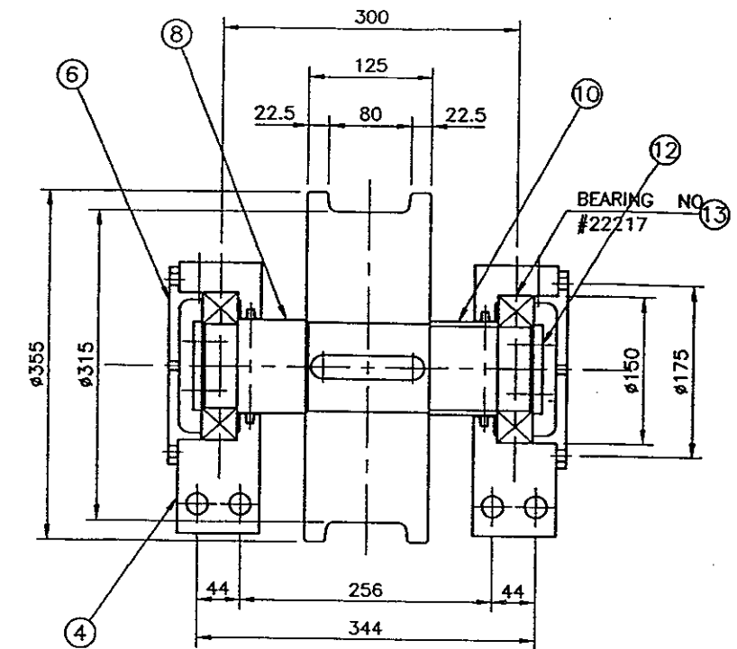
IDLE WHEEL ASS'Y
